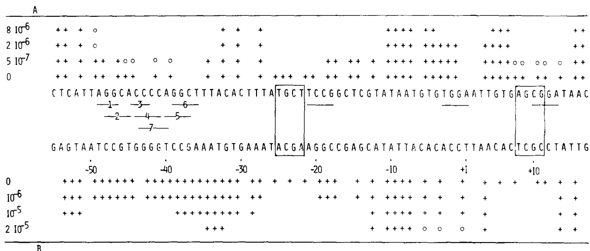
Fig. 3. Schematic representation of act D binding sites along the lac UV5 promoter-operator region. Asterisks indicate sites cut down by DNase I. Open circles denote sites where the digestion was partially inhibited by act D. Concentrations of act D are shown to the left. (A) Upper chain is labelled; DNA concentration 4 \mu\text{M} bp. (B) Lower chain is labelled; DNA concentration 0.8 \mu\text{M} bp. Consensus tetranucleotide - XCGY, where X \neq G and Y \neq C are boxed. Putative binding sites of act D molecules are underlined. Inserted numbers designate alternative putative binding sites discussed in the text.
