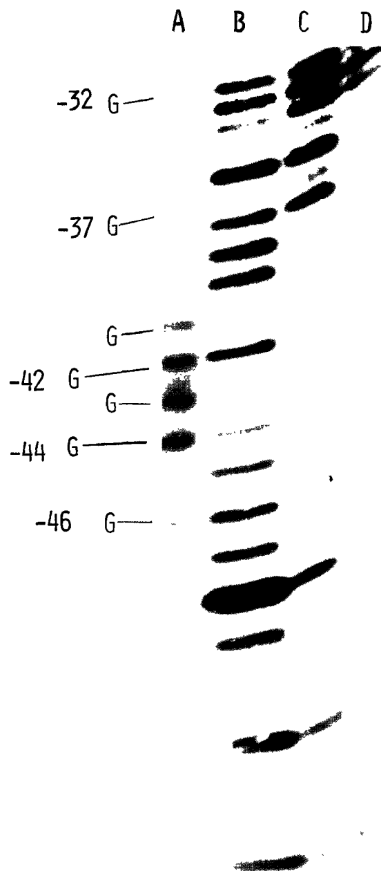
Fig.2. Cooperativity of act D-DNA binding. DNA concentration was 0.5 mg/l (0.8 \mu M nucleotide bp). Lower strain of DNA is labelled. Polyacrylamide concentration was 20%. (A) A + G dimethyl sulfate reaction; act D concentration: (B) 1 \mu M, (C) 10 \mu M, (D) 20 \mu M.
